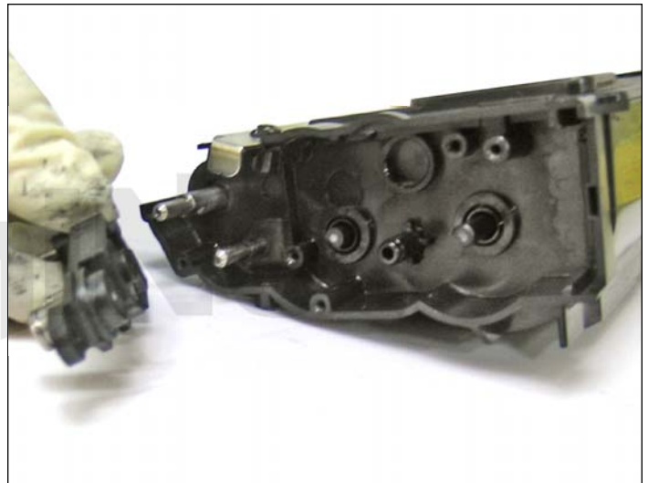
16. Gearside developer roller support removed.
