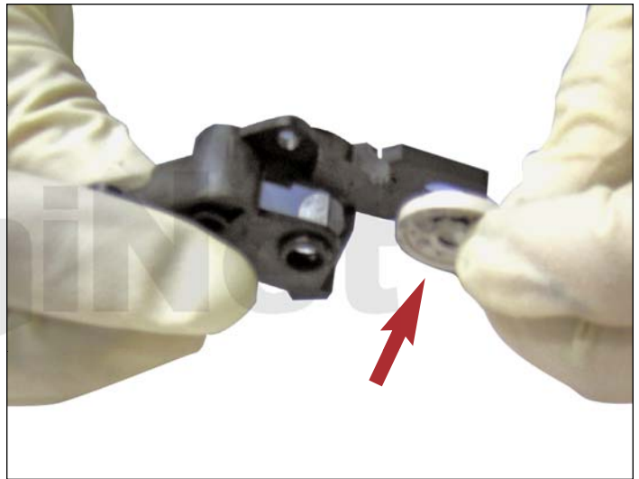
8. Gearless side developer roller support shown with bearing attached.
