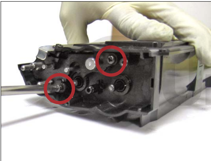
15. Remove the two developer roller support screws from the gearside of the cartridge.
