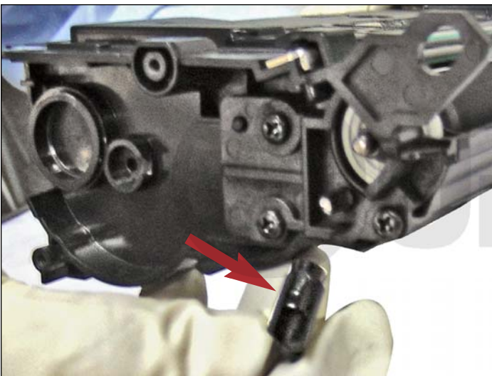
3. Remove the extension gear next to the developer roller on the gearless side of the toner cartridge.
