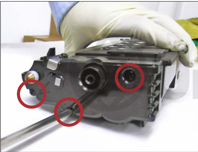
9. Remove the three gearside end cap screws shown.
