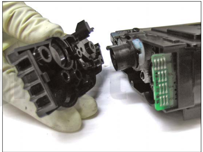
10. Remove the gearside end cap.
