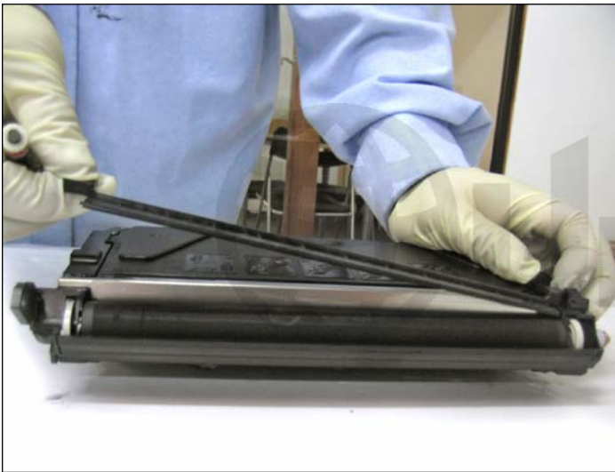
5. Lift up and remove the doctor blade cover in the direction indicated by the arrows shown.
