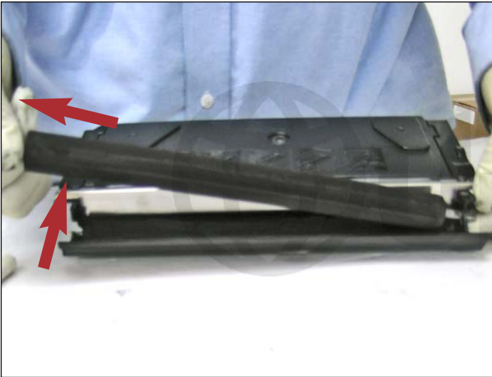
17. Lift up and pull out the developer roller in the manner shown.
