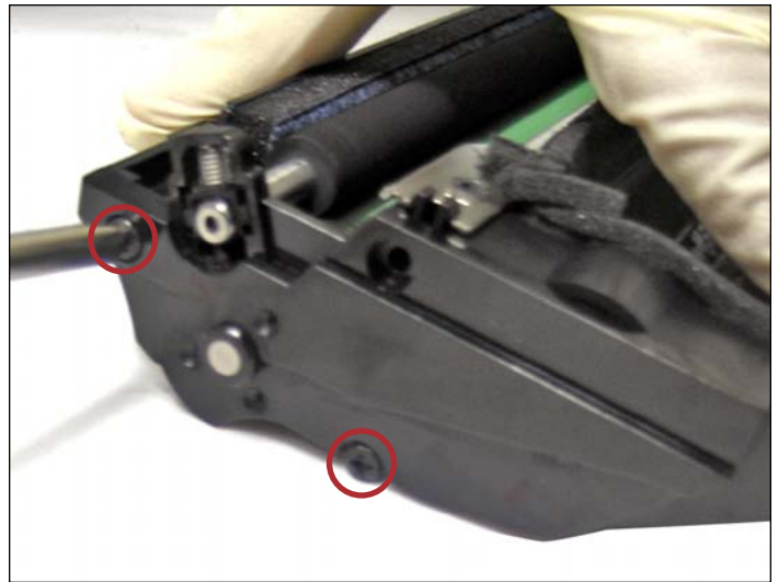
8. Remove the two screws indicated to release the gearside end cap.
