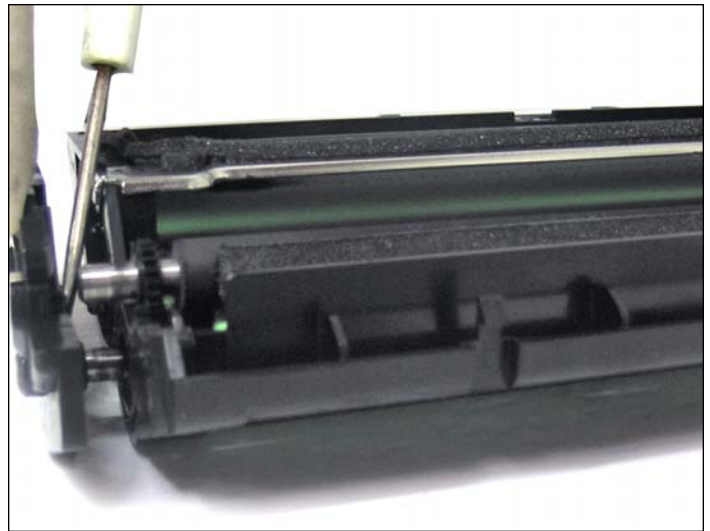
6. The end cap should slide out easily.
