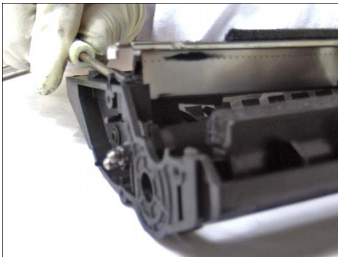
13. Once the foam seal is completely detached, you are then ready to remove the doctor blade.
