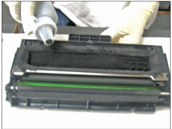
24. Refill toner before installing top cover.
