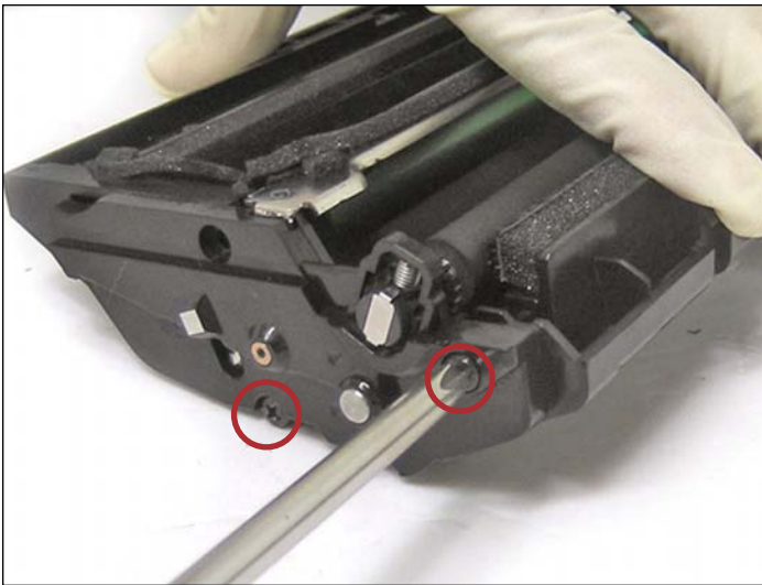
5. Remove the two indicated screws from the gearless side.
