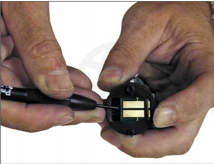
5. While pulling out on the top of the chip holder, slide the chip out with a small screwdriver. Replace the chip.
